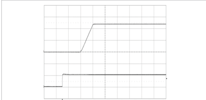
Start-up enabled by connecting V_1 at: T_{P1}, T_{P3} = +25^{\circ}\text{C}, V_1 = 53\text{ V}, I_O = 39\text{ A} resistive load. Top trace: output voltage (5 V/div.). Bottom trace: input voltage (50 V/div.). Time scale: (10 ms/div.).
