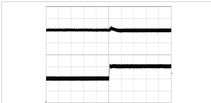
Output voltage response to input voltage transient at: T_{P1}, T_{P3} = +25^{\circ}\text{C}, V_1 = 40\text{-}60\text{ V}, I_O = 19.5\text{ A} resistive load, C_O = 3.9\text{ mF} Top trace: output voltage (2 V/div.). Bottom trace: input voltage (20 V/div.). Time scale: (0.5 ms/div.).
