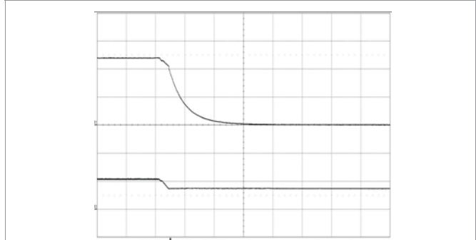
Shut-down enabled by disconnecting V_1 at: T_{P1}, T_{P3} = +25^{\circ}\text{C}, V_1 = 53\text{ V}, I_O = 39\text{ A} resistive load. Top trace: output voltage (5 V/div.). Bottom trace: input voltage (50 V/div.). Time scale: (2 ms/div.).
