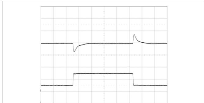
Output voltage response to load current step-change (9.75-29.25-9.75 A) at: T_{P1}, T_{P3} = +25^{\circ}\text{C}, V_1 = 53\text{ V}, C_O = 3.9\text{ mF}. Top trace: output voltage (0.5 V/div.). Bottom trace: output current (20 A/div.). Time scale: (0.5 ms/div.).
